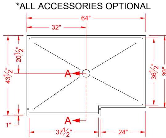
TOP VIEW - SCALE \frac{3}{8}" = 1'-0"
